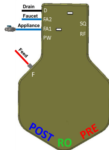
Figure 4: System Connections
