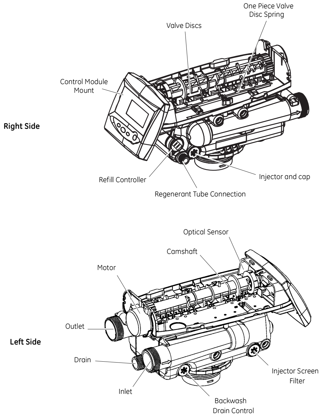
Figure 2 Performa Valve Identification
